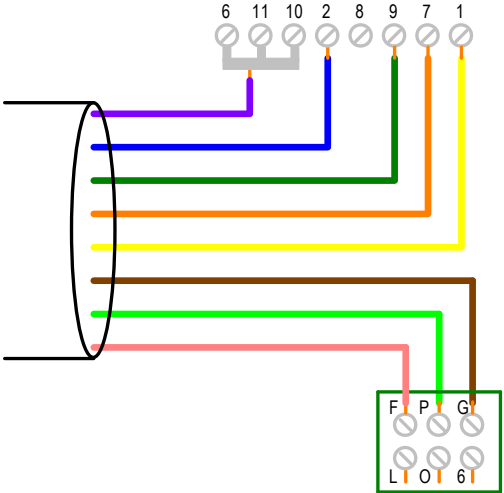
Old style 1130/NID handset connections
